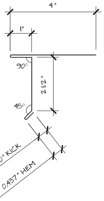
Closed Small Hem Eves Drip Bull Nose - 8.437"
