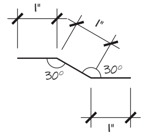
Valley Cleat - 3"
