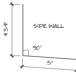
5x5 Flashing
